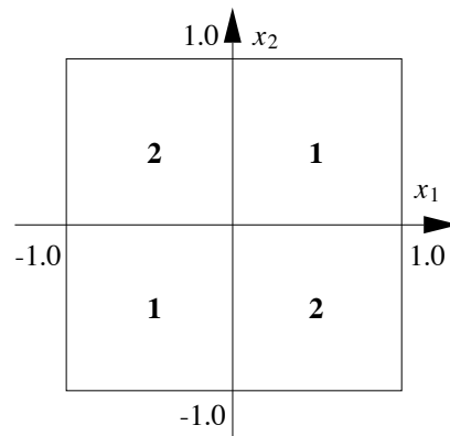
Fig. 8. Pseudo XOR problem: Regions occupied by the two non overlapping classes.
